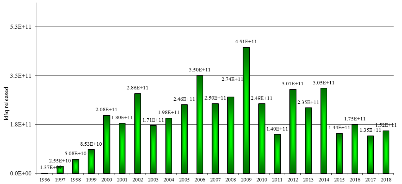
Tritium Gaseous Emissions UI - 1996 - 2018
