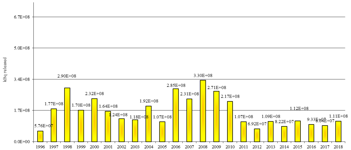
C-14 in Gaseous Emissions U1 1996 - 2018
