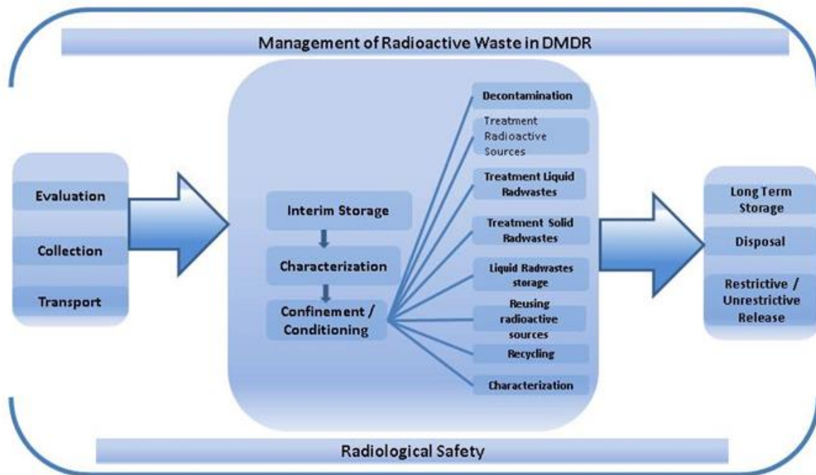
Figure B7: IFIN-HH Radioactive waste management scheme
