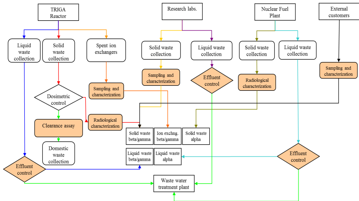
Figure B9: ICN Pitesti Radioactive Waste Management Scheme
